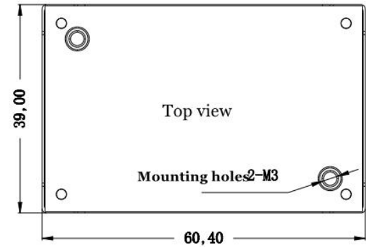
Standard 60.4*39*12.7mm
