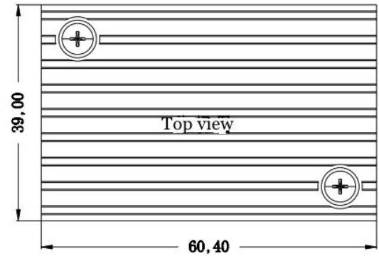
Standard+Heatsink 60.4*39*27.7mm
